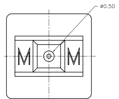
VIEW "Y"
