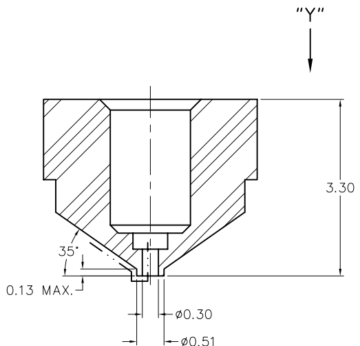
SECTION X-X
